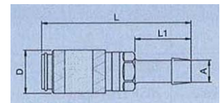
Hose stem
