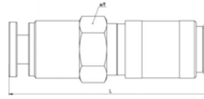
Push-in
